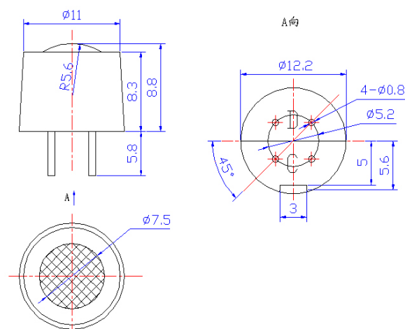
Fig1.Sensor Structure
