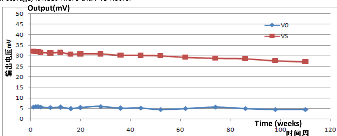
Fig10. Sensitivity fluctuation
