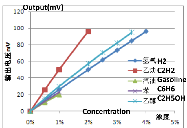
Fig3. Sensitivity Curve
