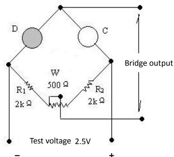
Fig1.Sensor Structure
